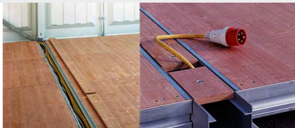
System cassette flooring with integrated cable channel and variable cable exit positioning
